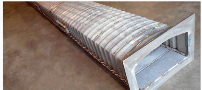
Corrugated Muffle with Stainless Steel Hearth Plates
